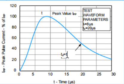
Fig1. 8/20μs Pulse Waveform
